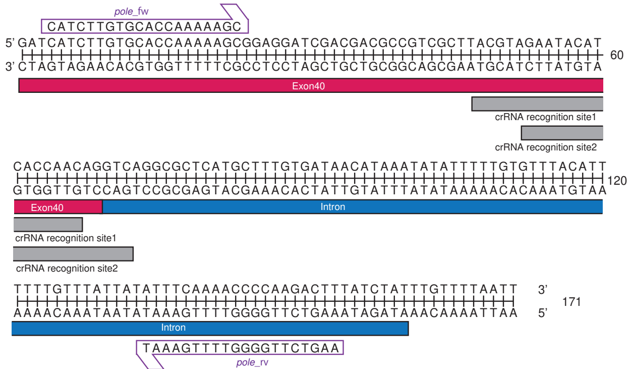
Suppl. Fig. 4: Partial sequence of pole , crRNA recognition sites 1 and 2, and primers for amplification of the target region.
