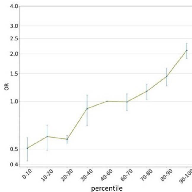
Figure 3 OR of BC risk as a function of BC PRS deciles. PRS was generated using Lassosum. OR is measured relative to scores in the middle PRS quintile (40%–60%). Shown are means and SEMs over the six holdout sets. BC, breast cancer; PRS, polygenic risk score.
