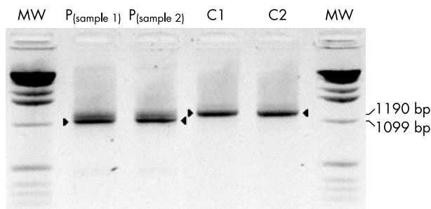
Figure 4 RT amplification of the FTSJ1 gene spanning the 11 coding exons. The amplification of the wildtype transcript results in a 1190 bp product (C1 and C2, lanes 4 and 5), while the transcript of the patient (P, IV-1; samples 1 and 2, lanes 2 and 3) is significantly shorter; it lacks exon 4 as demonstrated by cDNA sequencing (fig 3).
